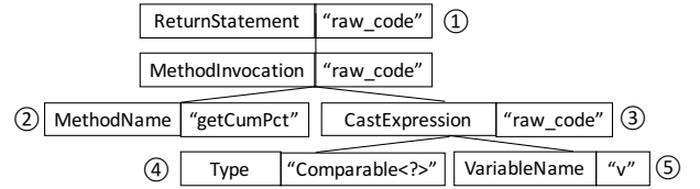
Figure 5: AST of bug Math-75 source code statement.
